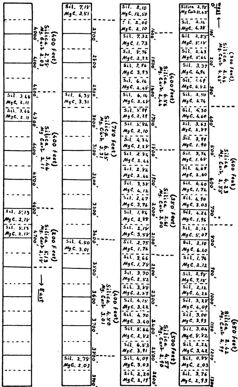
Figure 18. Diagram Cross-Sections showing the chemical composition of the Beekmantown Limestone along Potomac at Whiting's Neck.
